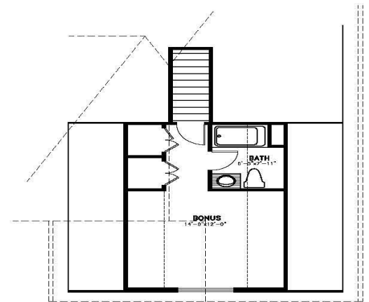
UPPER FLOOR PLAN 327 SQ.FT. UPPER FLOOR
